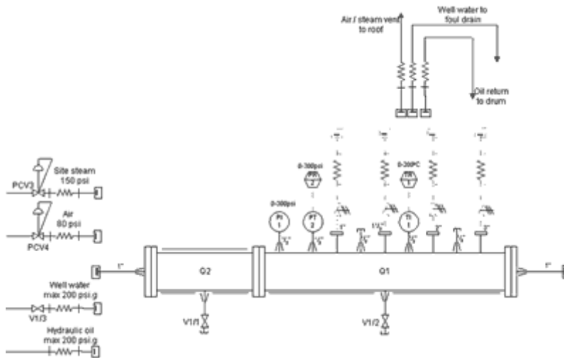
Figure 1 Schematic of the test rig (click image to enlarge):
