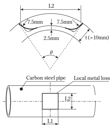
Fig. 4 Size of metal loss
