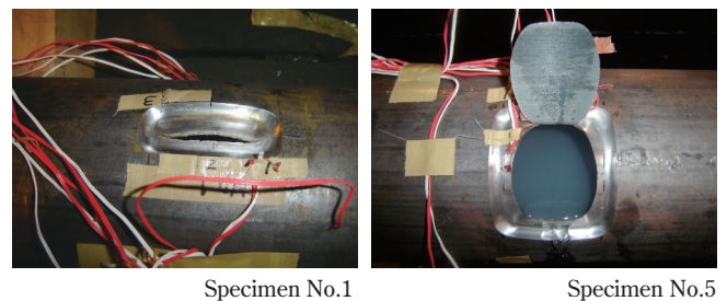
Fig. 6 Outer view of specimens after tests
